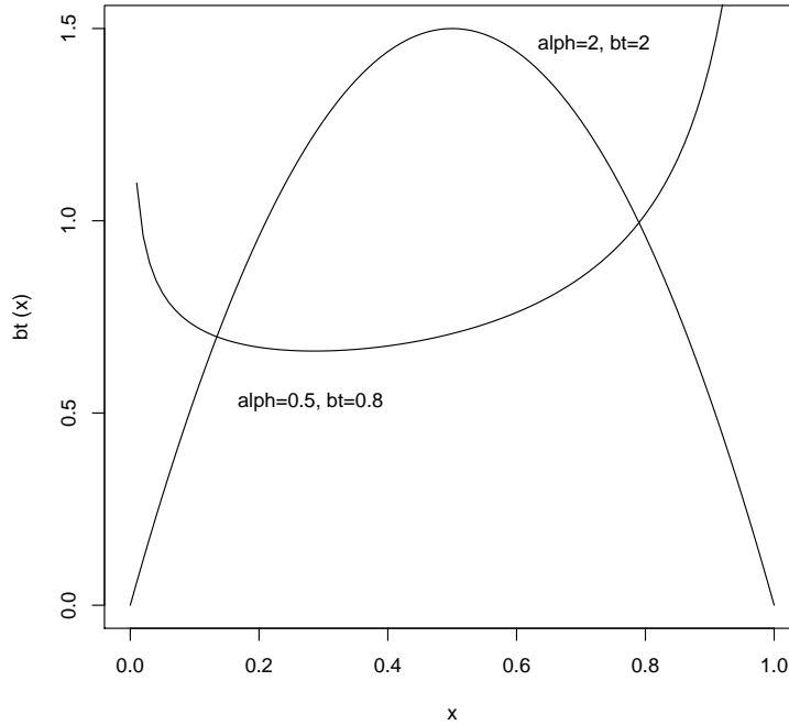
Figure 7.3: Two Beta Densities
